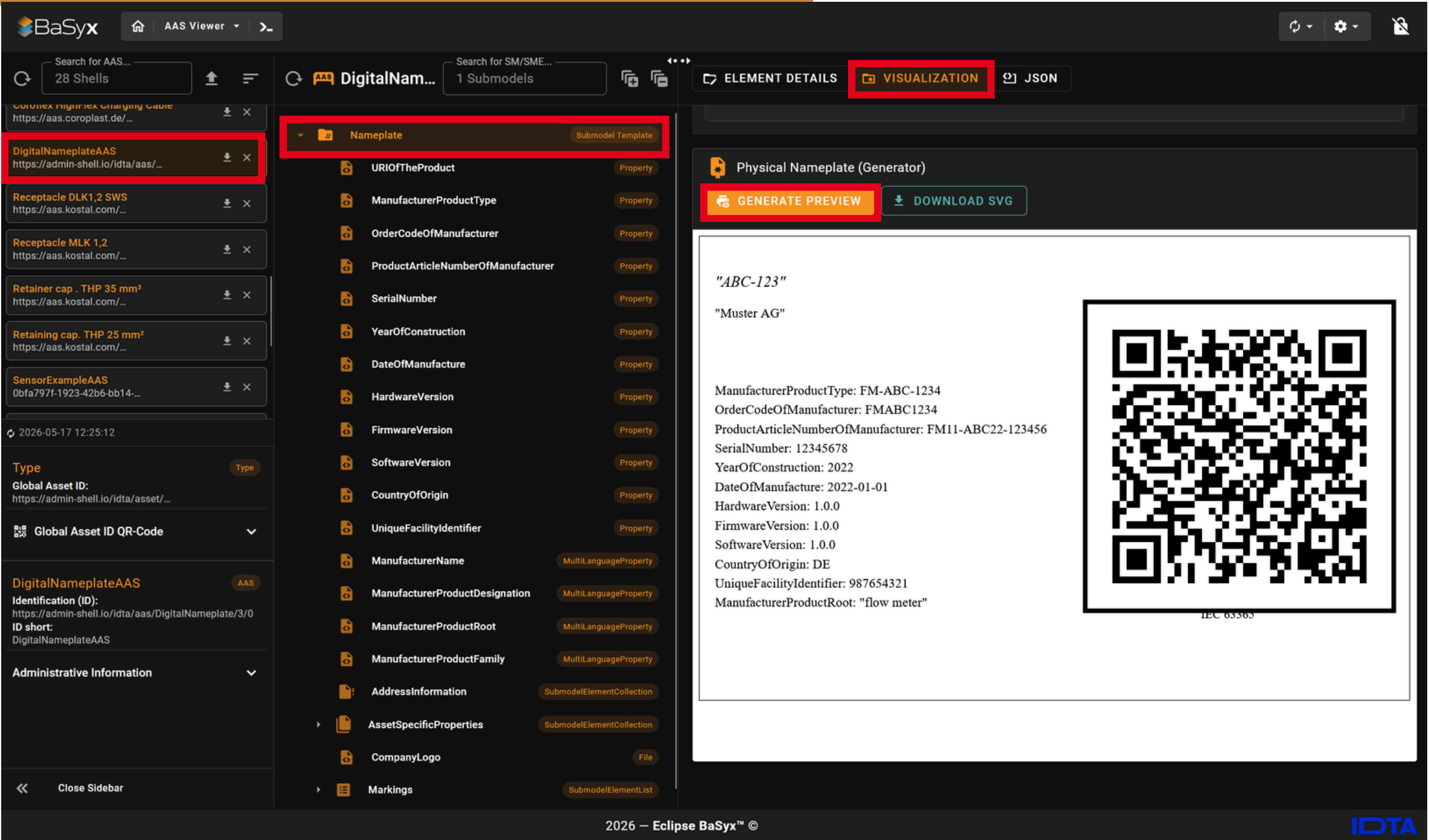
Fig. 8: Overview of BaSyx Viewer Nameplate
